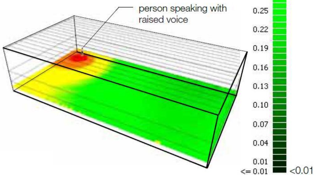
Speech intelligibility with 50 dBA ambient noise (some radiant heating systems)
