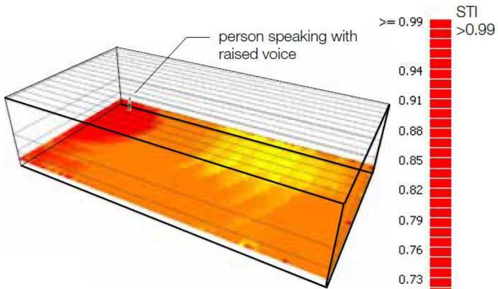
Speech intelligibility with low ambient noise
