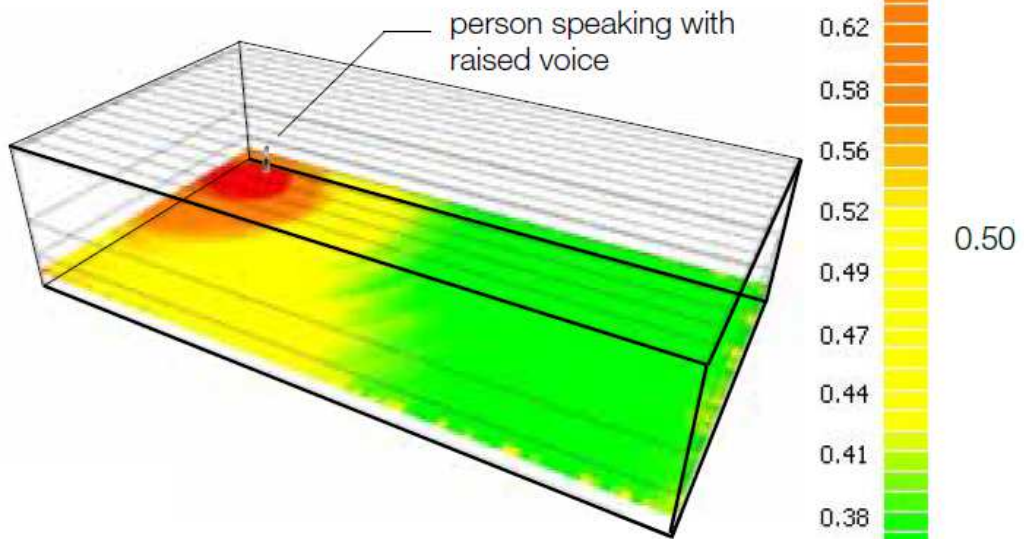
Speech intelligibility with 40dBA ambient noise (BB93 compliant)
